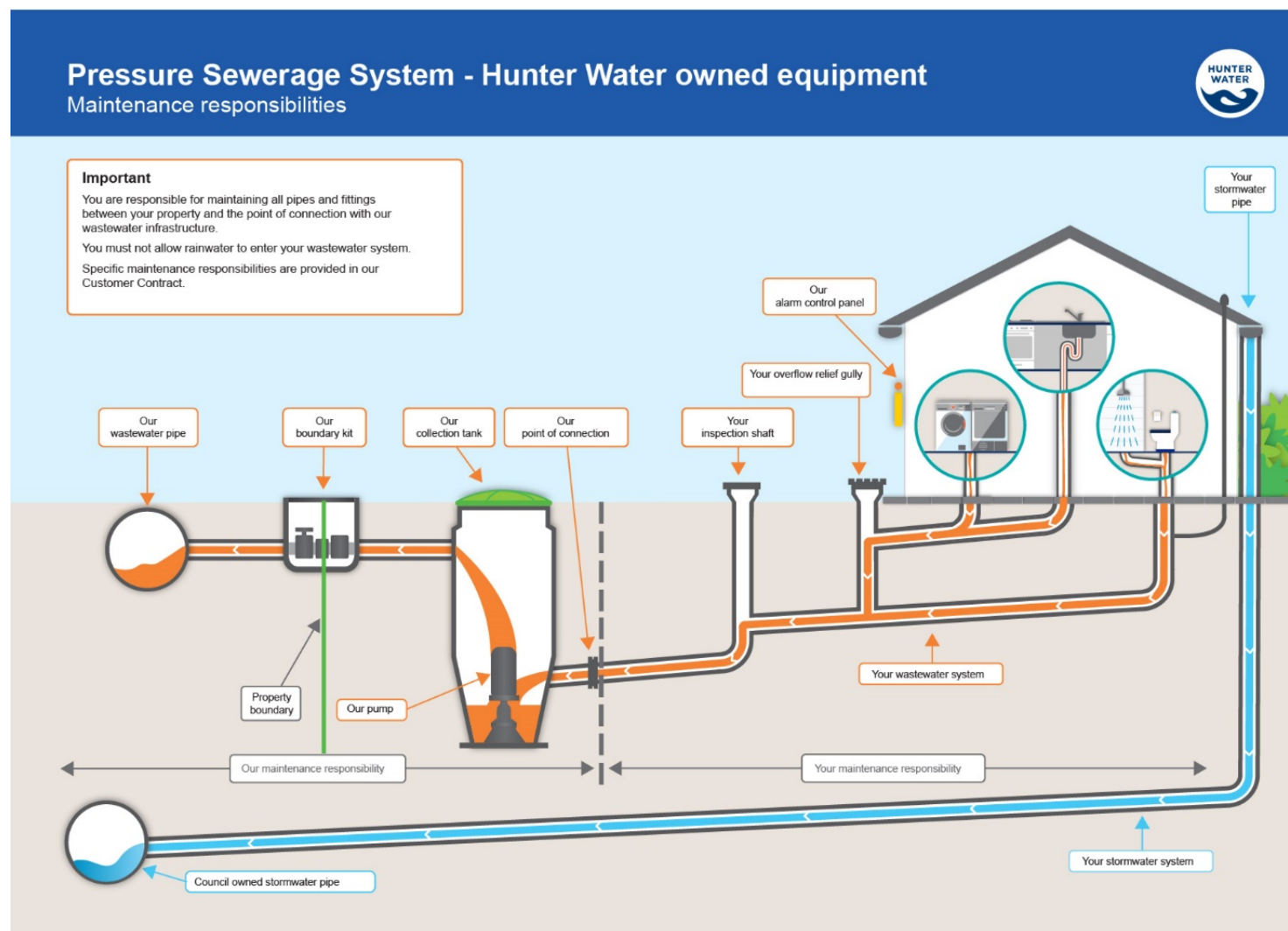
Figure 4 Typical Hunter Water pressure sewerage system (HWPSS) maintenance and responsibilities
