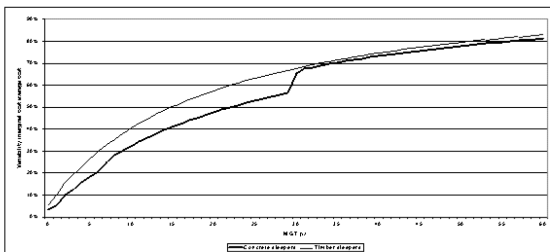
Figure 3.4 Variability of track life-cycle maintenance cost
