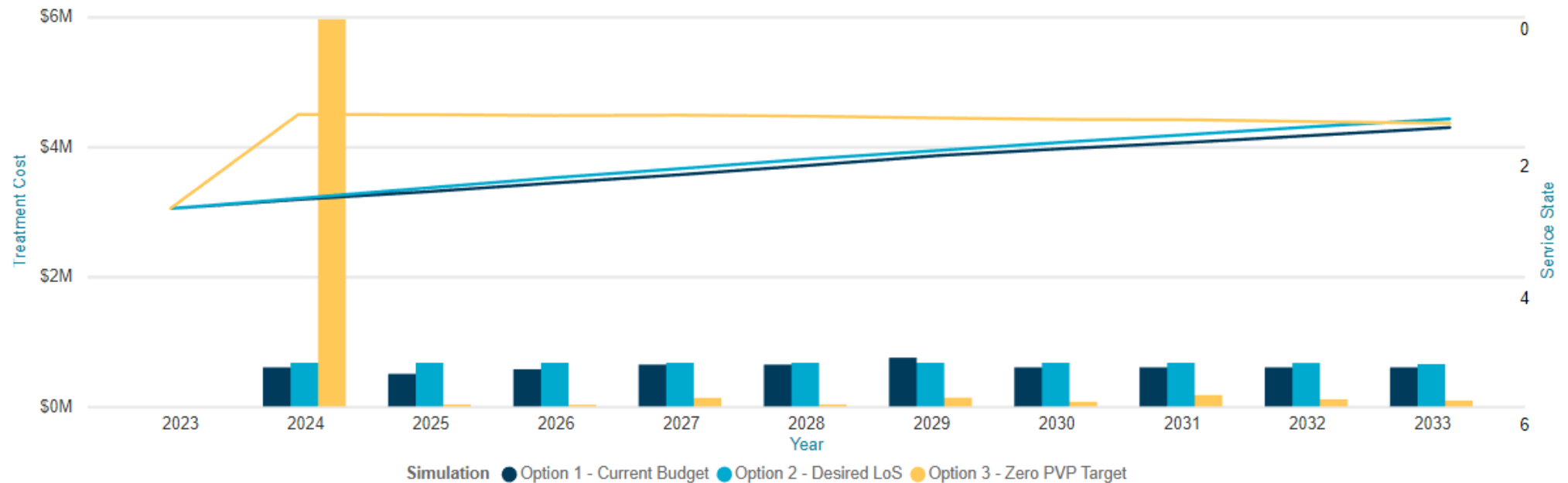
Figure 10b) Footpath Asset Class - Forecast 10-Year Capital Funding Analysis and Average Condition by Year
