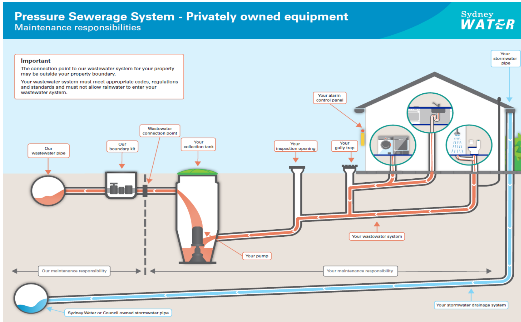
Figure 5: Typical Private Pressure Sewerage Equipment maintenance responsibilities
