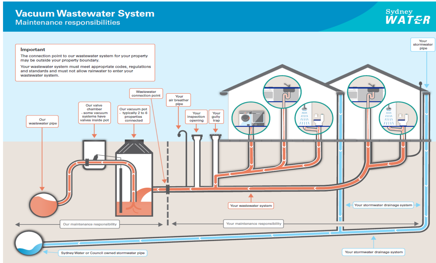
Figure 3: Typical wastewater system maintenance responsibilities – Vacuum wastewater system
