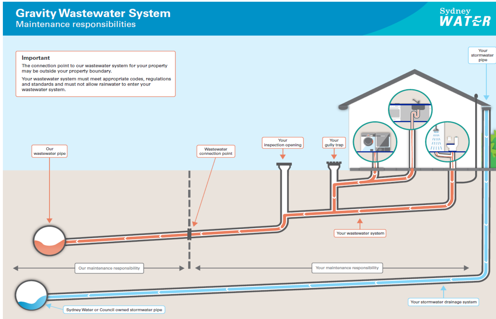
Figure 2: Typical wastewater system maintenance responsibilities – Gravity wastewater system
