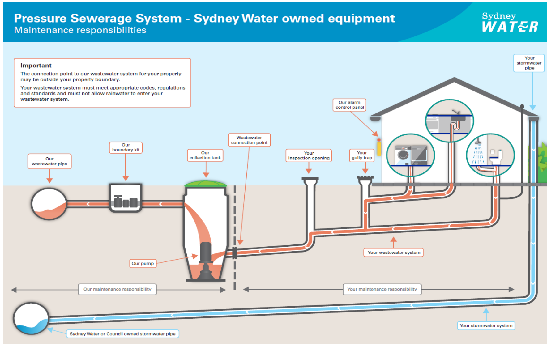
Figure 4: Typical Sydney Water Pressure Sewerage Equipment maintenance responsibilities
