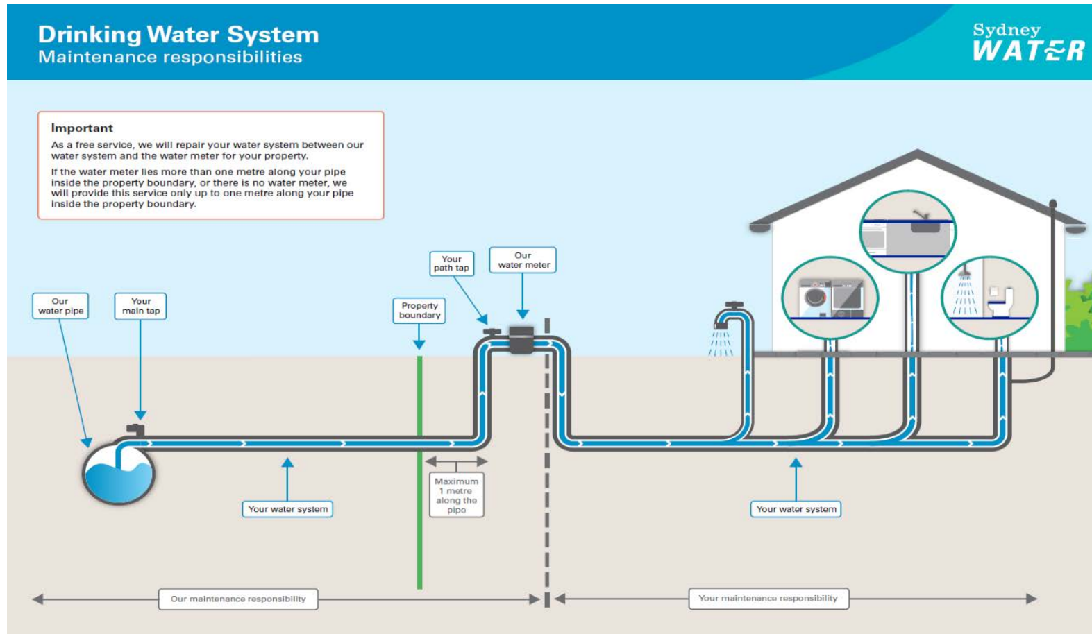
Figure 1: Typical water system maintenance responsibilities.
