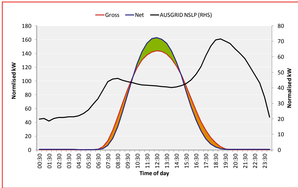
Figure 3: Normalised PV exports by interval
