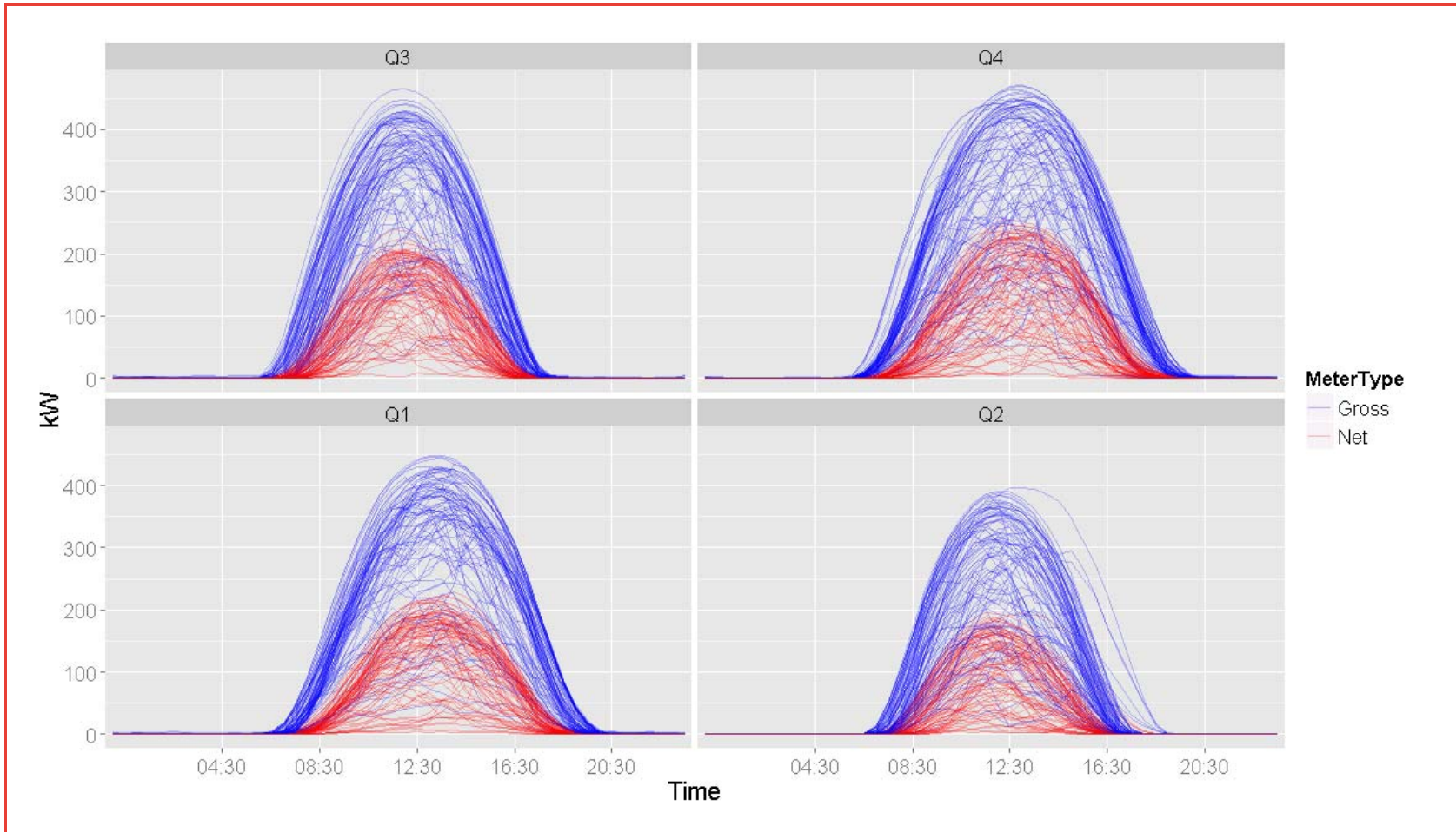
Figure 2: Diurnal PV export profiles – net and gross metered customers
