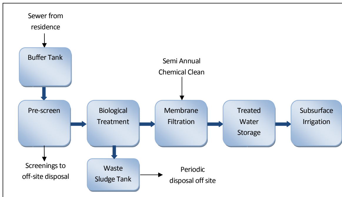
Figure 5.1 – Treatment process to achieve treated effluent fit for subsurface irrigation.
